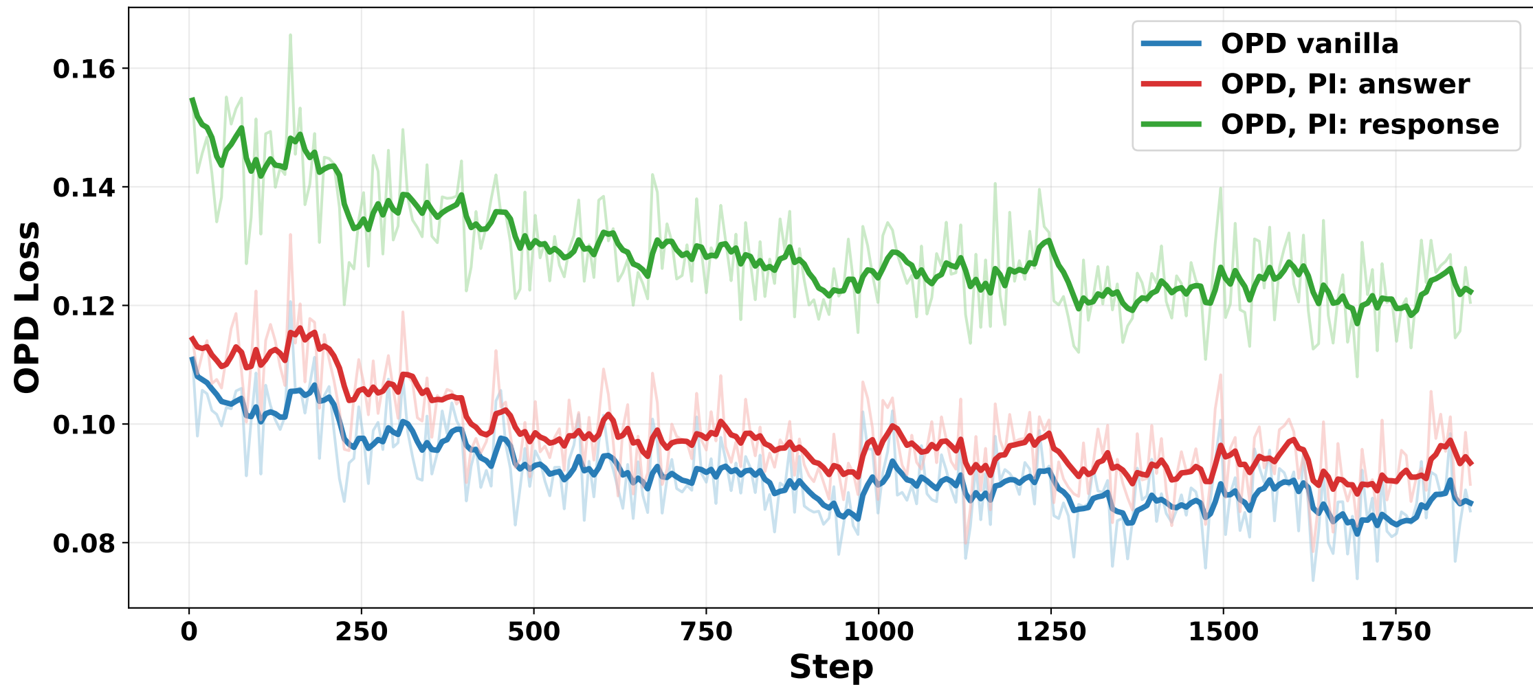
train/loss
